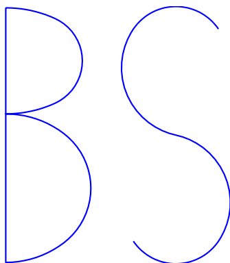
Two Letters Composed of Circular Arcs
